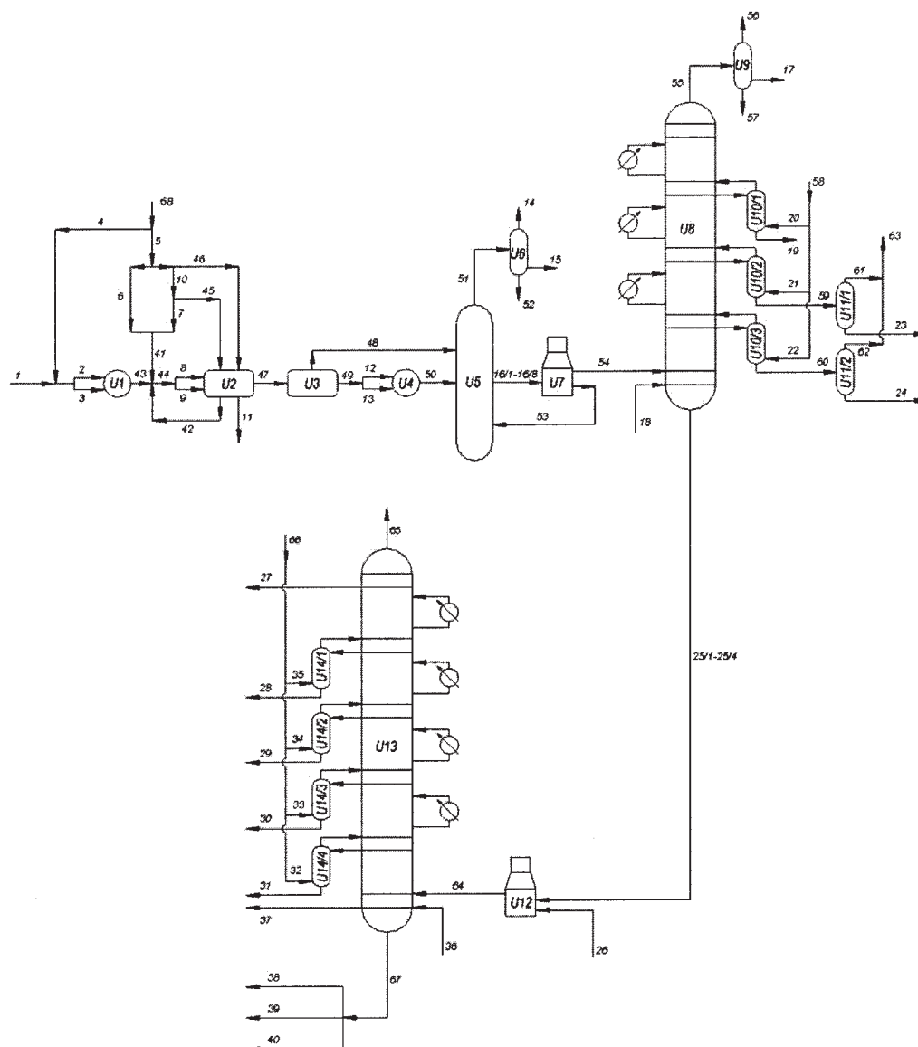
Figure 5. Flow sheet for crude distillation unit.
